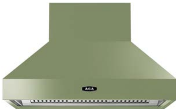
Olivine
